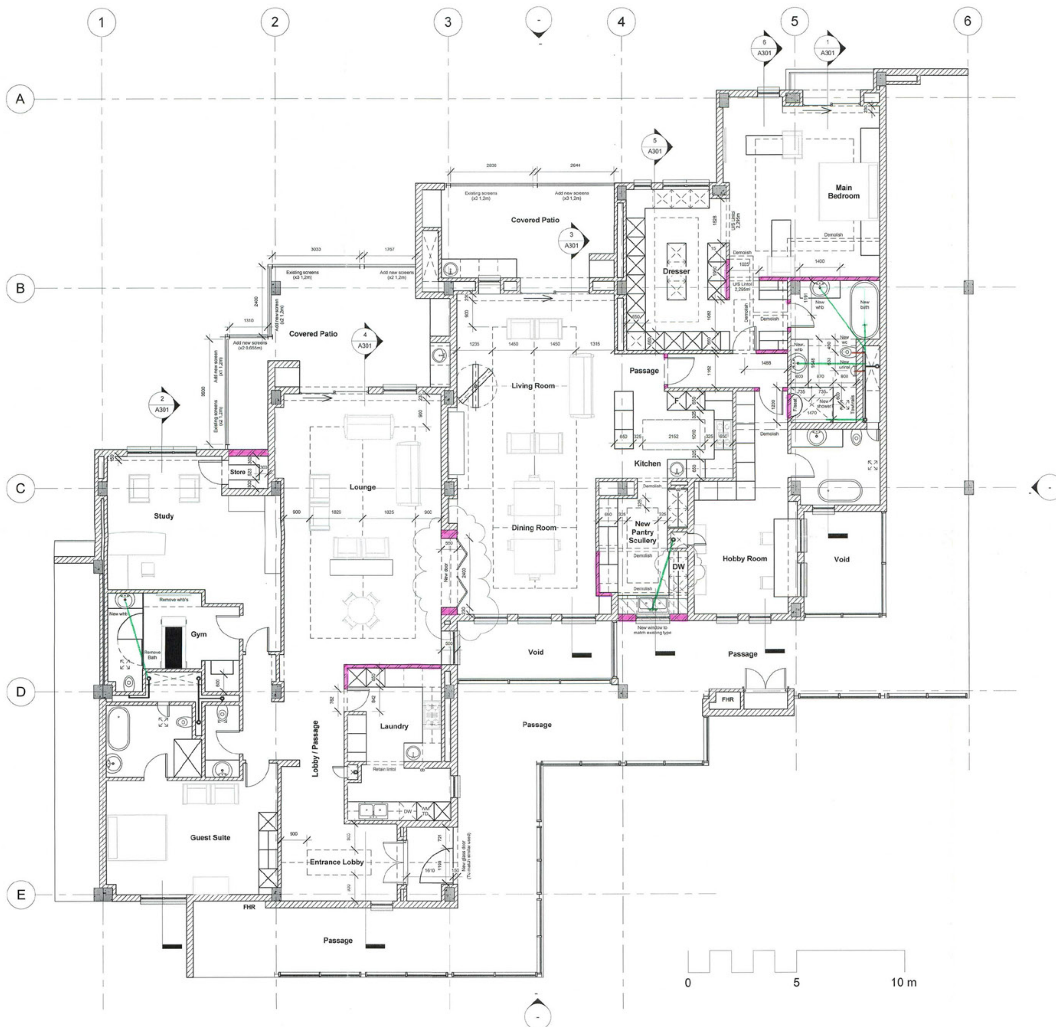
1 Level 1 Floor Layout (Unit 303 + Unit 304) 1:75
